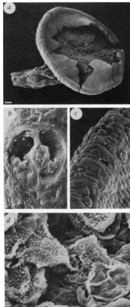
FIG. 1 Scanning electron microscopy (SEM; Cambridge microscope S360) of Cooksonia pertoni ssp. apiculispora , Gedinnian Shropshire (DE41). a, Complete specimen with short stalk (scale bar, 100 µm); b, stoma (scale bar, 5 µm); c, sporangial rim with papillate cells (scale bar, 30 µm); d, in situ spores from the dispersed taxon Streelispora newportensis , although this specimen lacks the characteristic proximal folding (scale bar, 5 µm).
