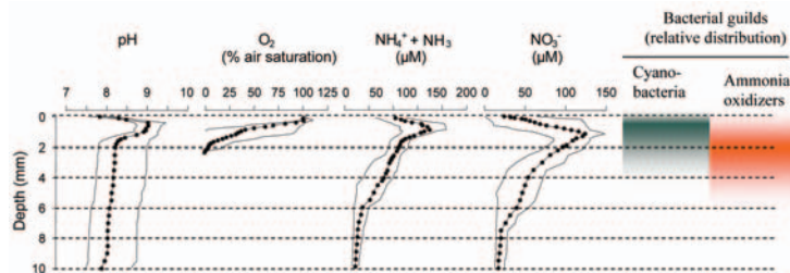
FIGURE 2 Chemical gradients in an active (wet) biological soil crust. Microelectrodes reveal microbial metabolic activity. Photoautotrophic cyanobacteria close to the surface consume CO 2 , driving pH up and creating an internal O 2 supply, which is quickly respired by heterotrophs leading to anoxia 2–3 mm below surface. Leakage of cellular NH 3 produced by cyanobacteria during N 2 fixation creates a thin layer with both free NH 3 and O 2 , which provides a habitat for chemolithoautotrophic ammonia-oxidizing bacteria. These provide nitrate through metabolism. These microscale processes provide the mechanistic basis for the fertilizing role of soil crust communities in arid lands at landscape scale (Garcia-Pichel et al. 2003).
