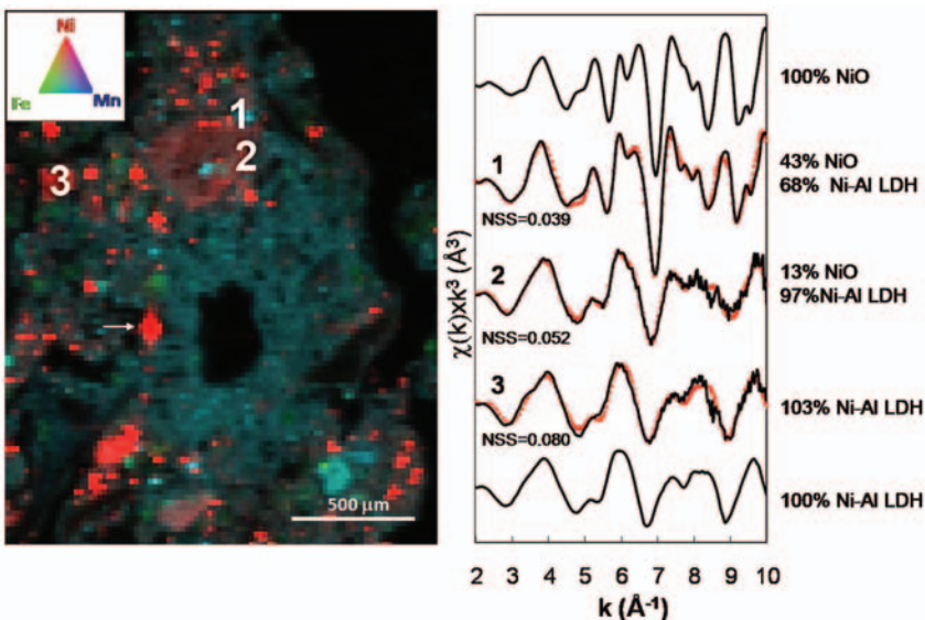
FIGURE 4 Weathering of \text{NiO}_{(s)} (at arrow) to form Ni-Al LDH in a smelter-impacted soil: (left) \mu -SXRF tricolor map of the Welland loam unlimed soil and (right) \mu -XAFS spectra from selected points within the map that show an increasing predominance of Ni-Al LDH relative to \text{NiO}_{(s)} resulting from progressive weathering (numbers 1–3). Solid lines represent the k^3 weighted \chi -spectra, and the dotted lines are best fits obtained using linear combinations fitting with NiO and Ni-Al LDH references (top and bottom spectra) (McNear et al. 2007).
