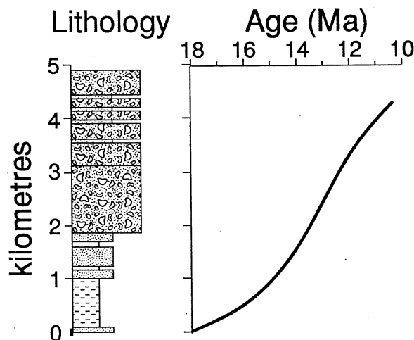
Fig. 1 Generalized lithological section at Las Juntas, Argentina with calculated sediment accumulation rates corrected for compaction. Lithologies are simplified to show dominant intervals of conglomerate, sandstone (stipple) and siltstone/mudstone (dashed). Data from Reynolds et al. (1990). Sedimentation rates are constrained by about 30 magnetic polarity reversals.
