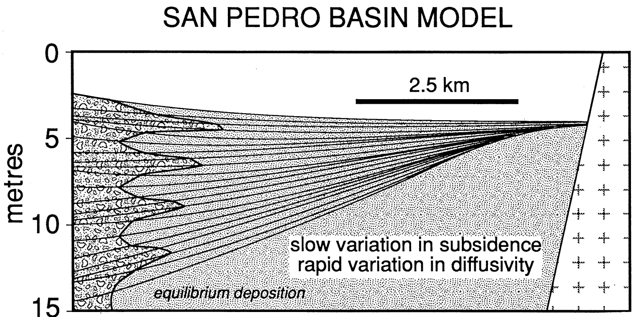
Fig. 4 Model result for gravel progradation into an asymmetric basin undergoing rapid variation in diffusivity superimposed on an overall slow decrease in subsidence rates. Time lines are drawn every 5 \times 10^4 yr. Symbols as in Fig. 1. Sediment derived from the left; subsidence is asymmetric, increasing to the left. Values used for model run are: T_{eq} = 5 \times 10^5 yr; n = 2 \times 10^{-4} km 2 yr -1 ; basin length = 10 km; subsidence rate = average sedimentation rate = 0.03 km 2 Myr -1 ; gravel fraction = 30% of total sediment supply; capture ratio = 0.9; diffusivity varies by an amplitude of 0.5 and cycles over a time period of 10^5 yr; subsidence varies by an amplitude of 0.8 and cycles over a time period of 2 \times 10^6 yr. See Part 1 for explanation of variables used in the model.
