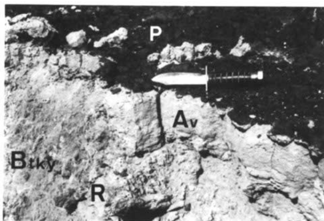
Figure 2. Stone pavement (P) formed over accretionary mantle in topographic depression on late Pleistocene flow in Cima volcanic field. Development of vesicular A ( A_v ) horizons of phase 1 soils, carbonate- and gypsum-bearing argillic horizons (Btky) of phase 2 soils, and origin of basalt rubble (R) are discussed in text.
