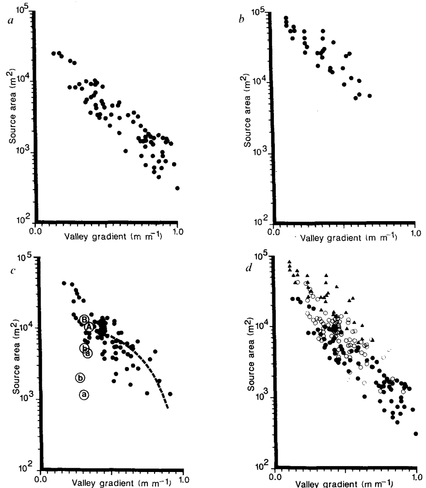
Fig. 1 Source area plotted against the local valley gradient, or slope at channel heads, \tan \theta , for a, Coos Bay, Oregon, b, southern Sierra Nevada, California, and c, Marin County, California. For the study area in c, downslope from the drainage divide in two hollows the slope within the source area is relatively constant (lower case letters in open circles) until the channel begins (capital letters in open circles). The dashed line is the relationship predicted by equation (1). d, Combined data from all three field areas, defining a strong inverse linear relation over the full range of data. The southern Sierra data (triangles) generally overlie the Marin County data (open circles) which, in turn, appear to overlie the Coos Bay data (solid circles). This difference is most clearly expressed in the low gradient sites.
