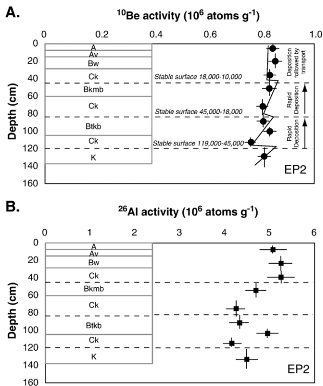
Figure 7. ^{10}\text{Be} data (A) and ^{26}\text{Al} data (B) for pit EP2. Nuclide activity neither increases nor decreases systematically with depth. Data points represent mid-point of depth interval. Vertical error bars represent sample depth interval. Horizontal error bars represent 1\sigma analytical uncertainty. Black line shows model fit explained in text. Dashed lines represent buried soil horizons. Number range represents period of stability in years before present. Soil data explained further in Table 1.
