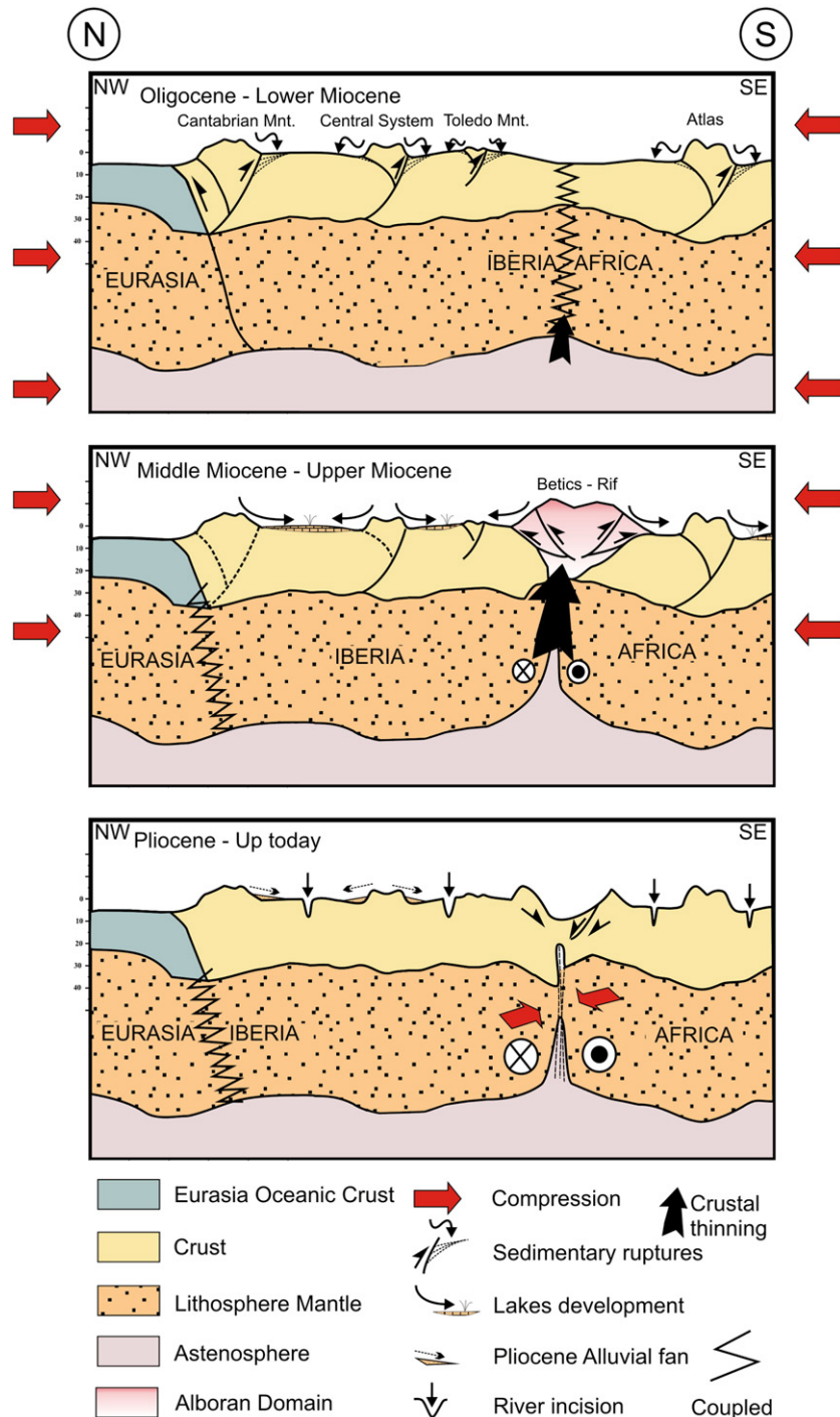
Fig. 16. Cross section sketches (not to scale) of the tectonic evolution of Eurasia–Iberia–Africa during the Cenozoic. Decoupling between Iberia and Africa is driven by the westwards displacement of the Alboran–Betics–Rif Block.
