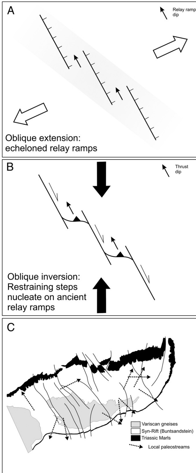
Fig. 13. A), B) Sketches showing how the nucleation of Cenozoic folds is located on ancient relay ramps and accommodation zones of the Triassic Rifting. C) Geological map of the Riba de Santiuste anticline with paleo-currents related to the Triassic infilling, indicating that the fold nucleation occurred on a sedimentation paleo-high (Sanchez-Moya, 1992) (Shown on Fig. 10a).
