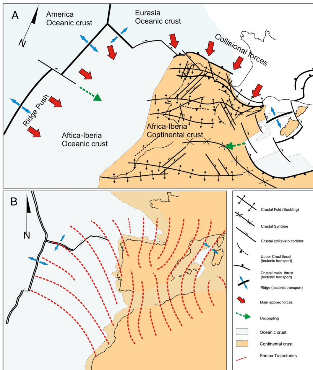
Fig. 3. A) Paleoplates sketch for Lithospheric folding development. B) Paleostresses reconstruction, we take S_{\text{hmin}} at the Ridge as ridge push to join with S_{\text{hmax}} . (30–20 Ma) Oligocene–Lower Miocene.
