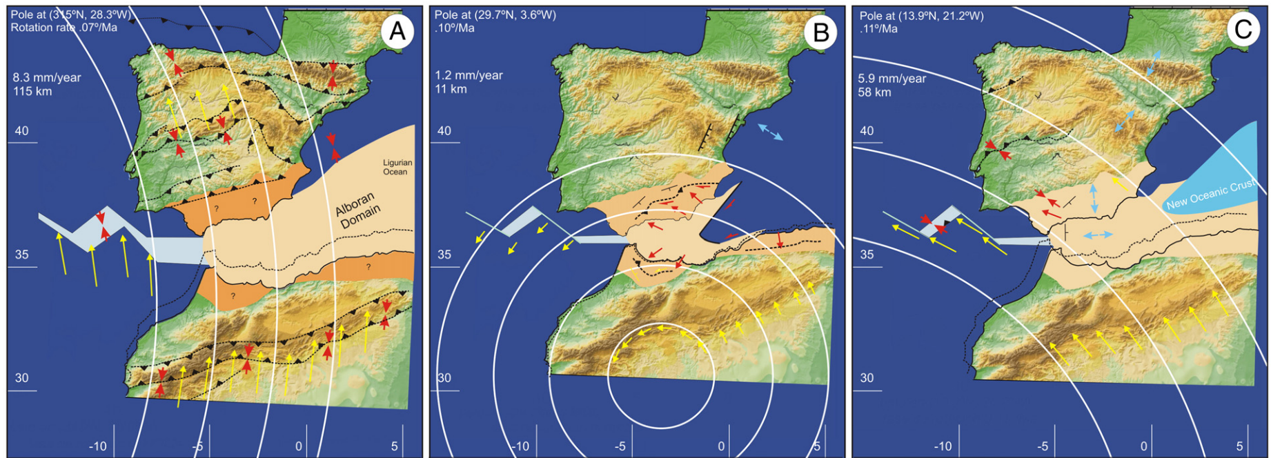
Fig. 2. Paleopoles of Iberia-Africa movement during the Cenozoic. Modified from Rosenbaum et al. (2002). A) Relative Africa-Iberia movement between An 13 and An 6: Iberia moored to Africa. B) Relative movement between Africa-Iberia An 6 and An 5: Iberia-Africa decoupling. C) Relative movement between Africa-Iberia An 5 and Present day. Iberia is a part of Eurasia. Red arrows: Shortening. Blue arrows: Extension. Yellow arrows: mean displacements.
